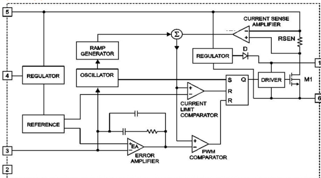
Figure1 Function Block Diagram of EC1466
