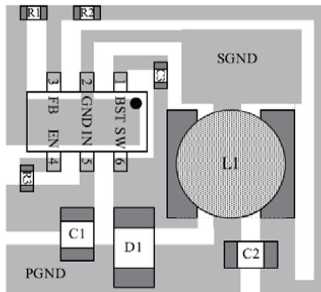
Figure 2: PCB Layout
