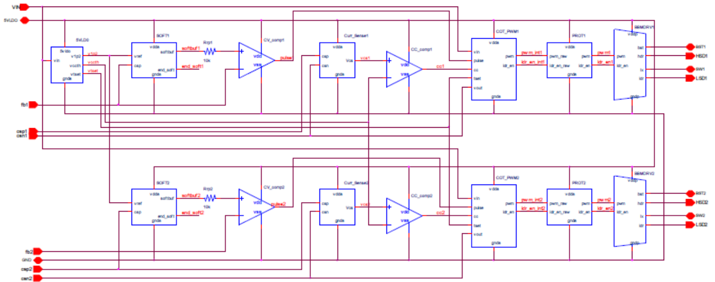
Figure 2 Function Block Diagram of EC1742
