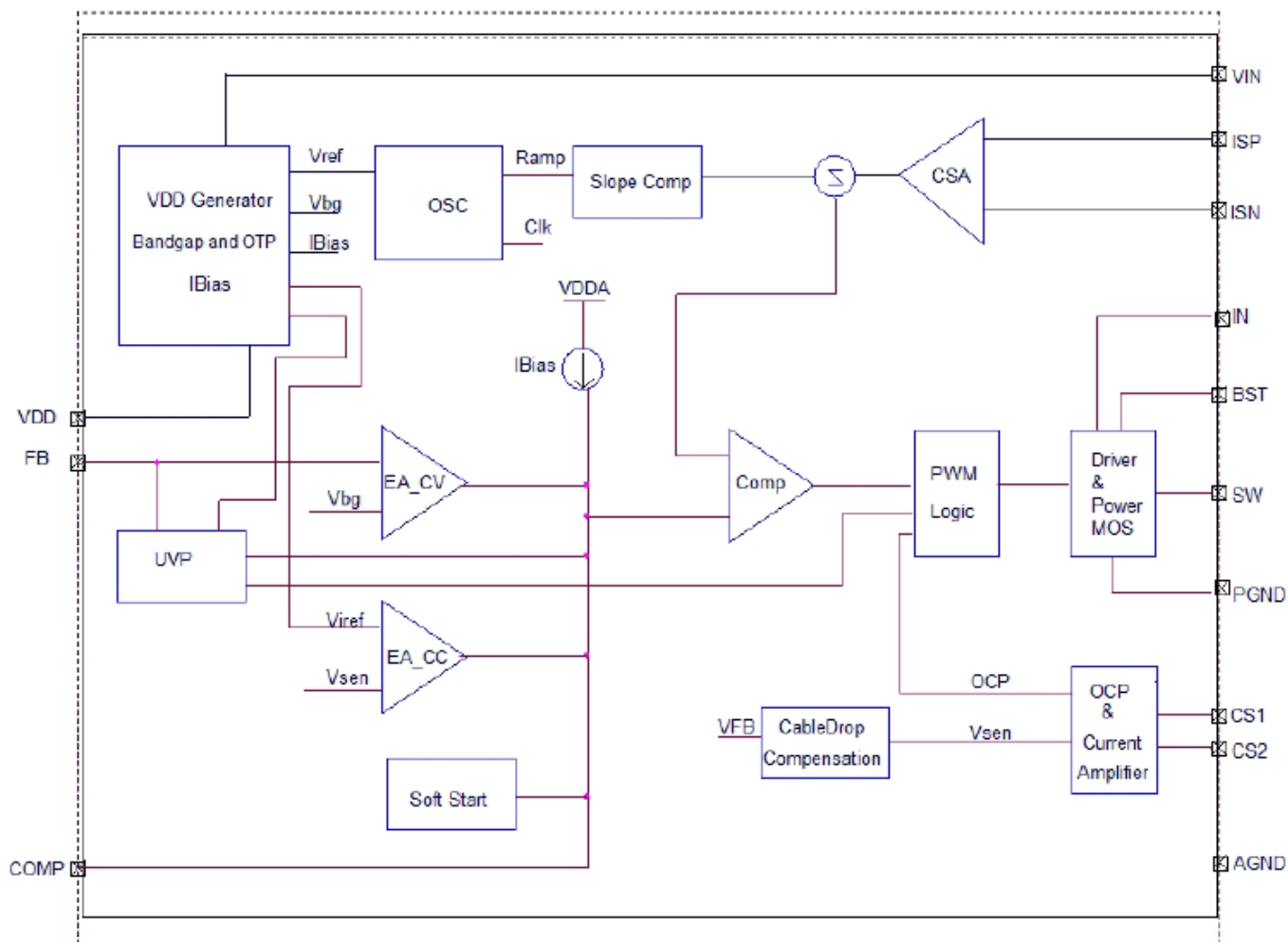
Figure 2 Function Block Diagram of EC1745
