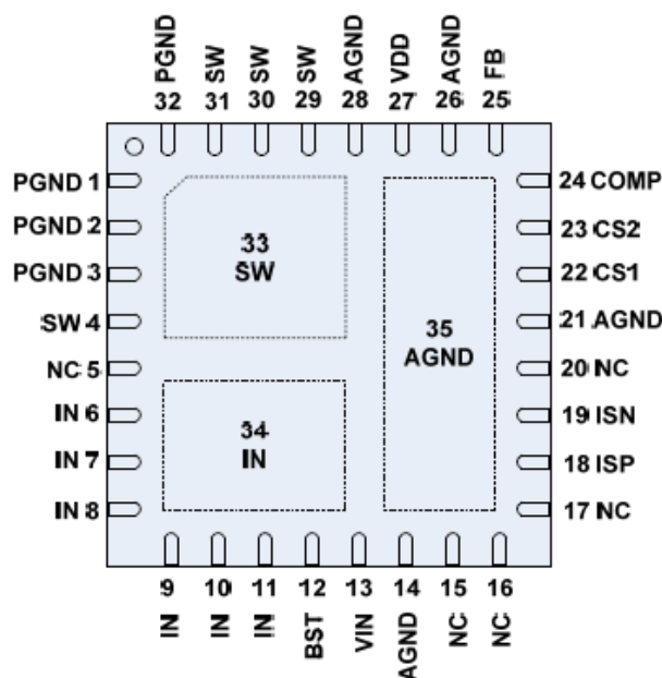
Figure1 Pin Configuration of EC1745(Top View)
