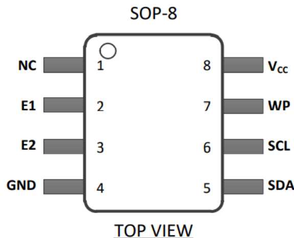
Figure 1–1 Pin Configuration
