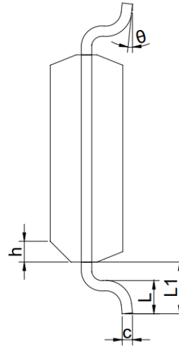
END VIEW
