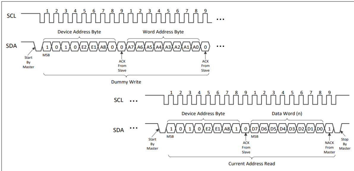
Figure 5–11 Random Read
