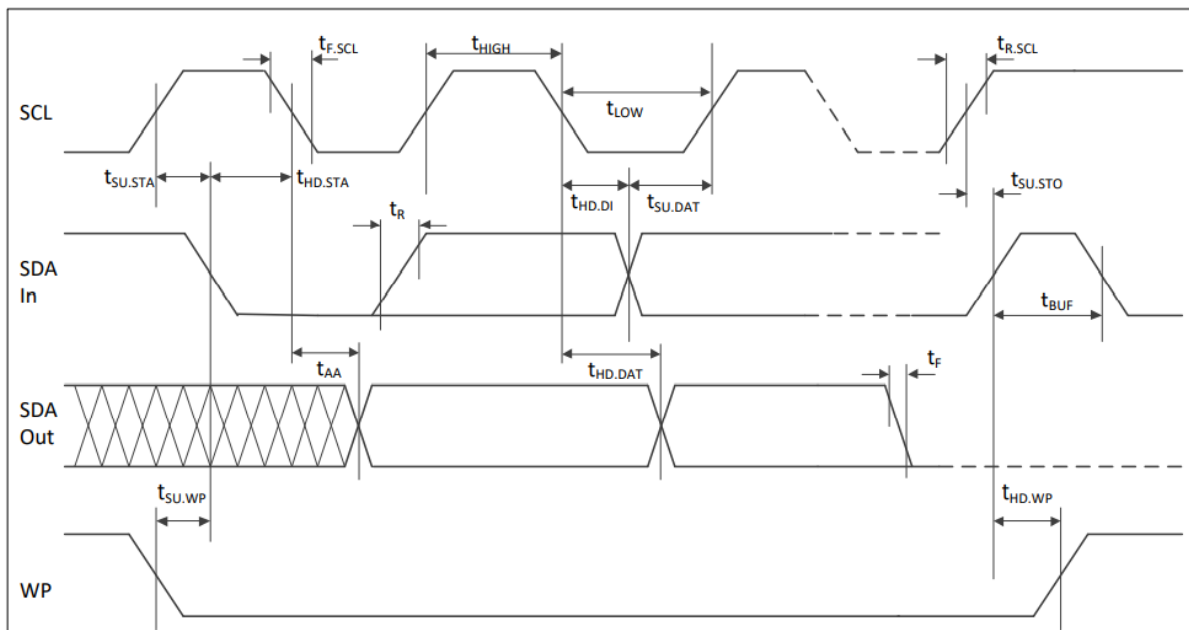
Figure 6-1 Bus Timing
