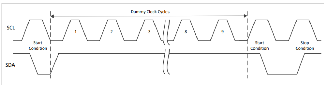
Figure 3–2 2-wire Software Reset
