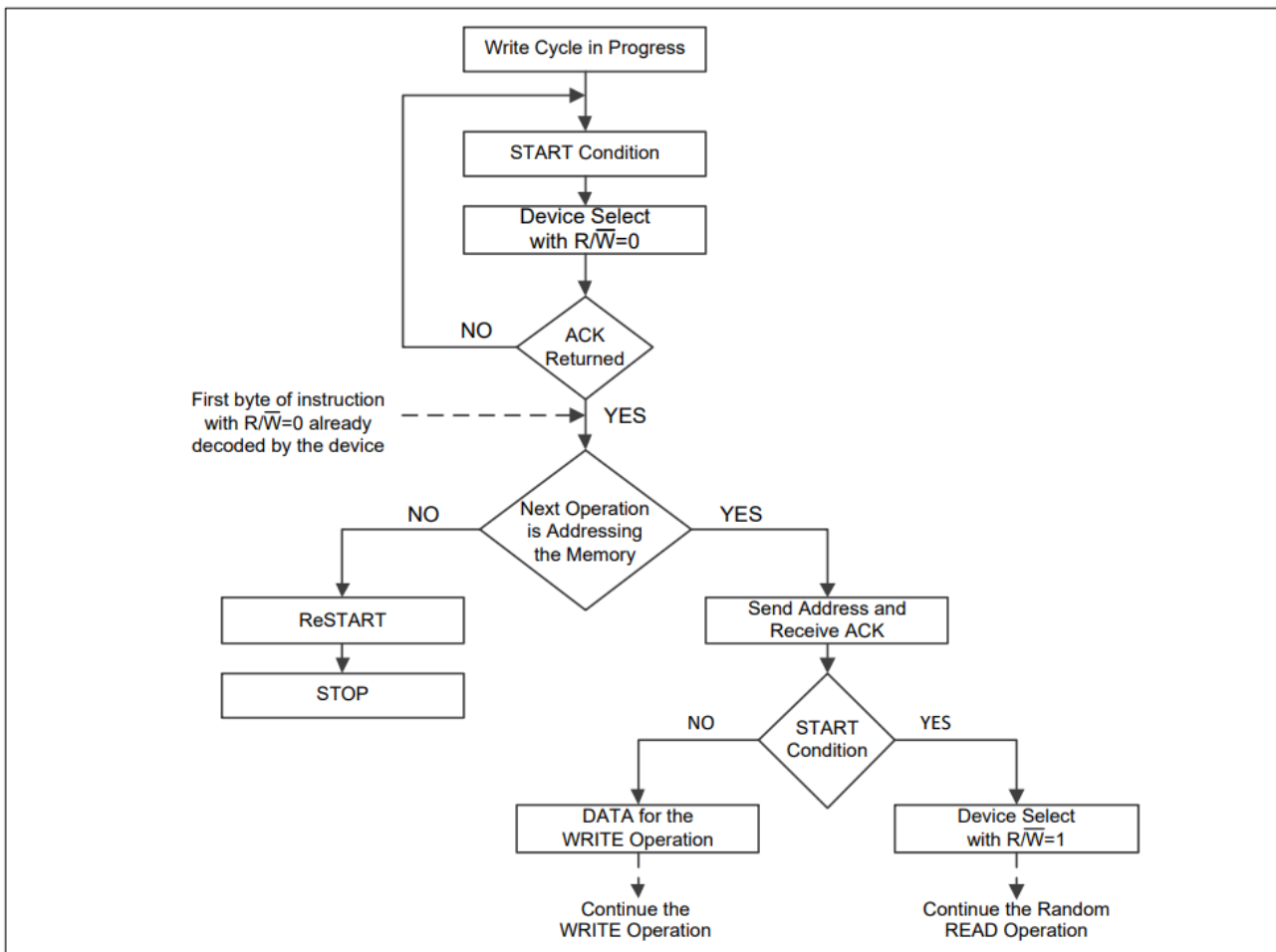
Figure 5-6 Acknowledge Polling Flow Chart
