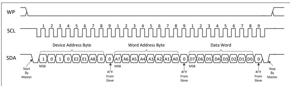
Figure 5–2 Byte Write Operation with Write Protection Pin Set to High (or SWP bit = 1)
