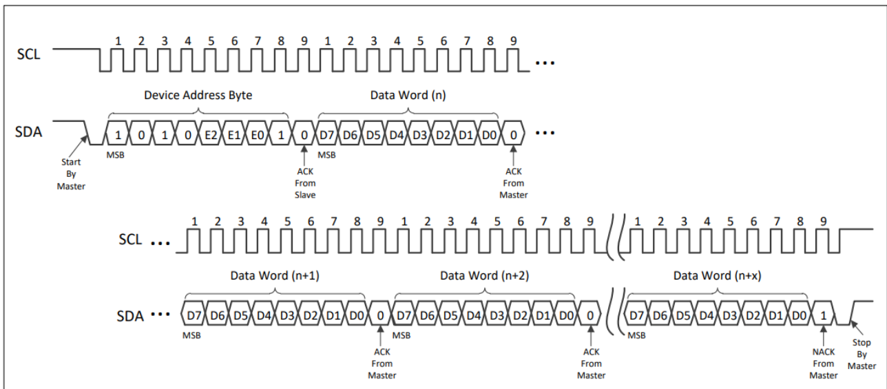
Figure 5–12 Sequential Read
