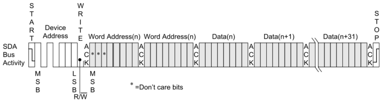
Figure 7. Page Write
