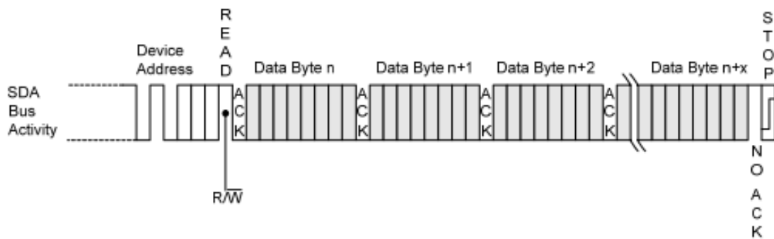
Figure 10. Sequential Read
