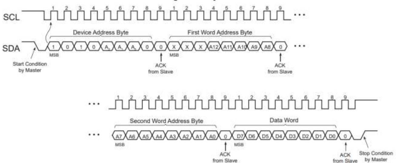
Figure 5-1. Byte Write
