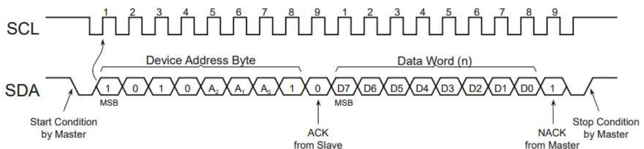
Figure 6-1. Current Address Read
