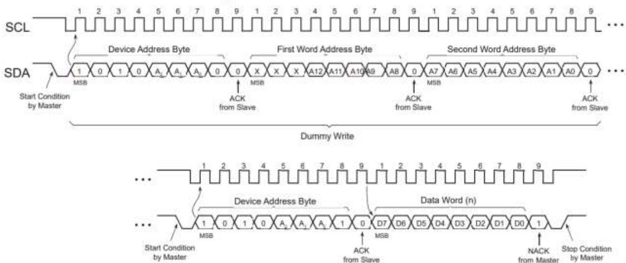
Figure 6-2. Random Read
