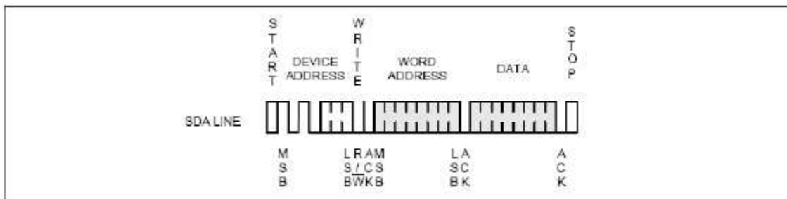
Figure 5: Byte Write
