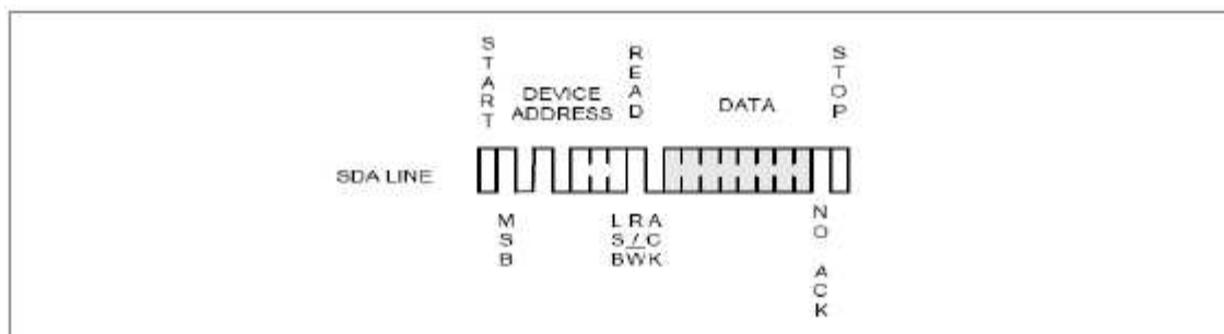
Figure 8: Random Read
