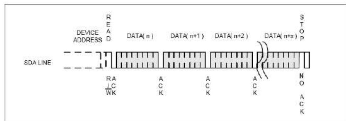
Figure 9: Sequential Read
