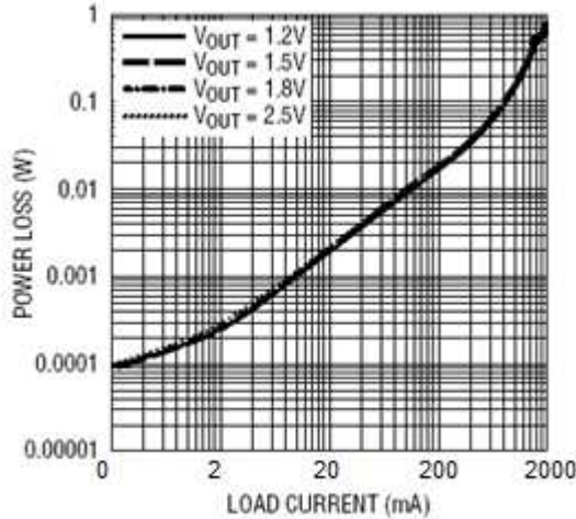
Figure 6: Power Lost VS Load Current
