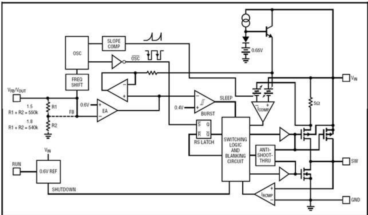
Figure2:Functional Block Diagram of EC3217
