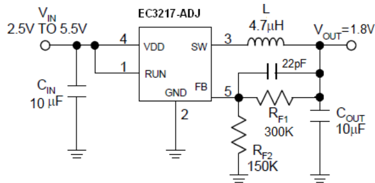
Figure 3. Type Application Circuit of EC3217
