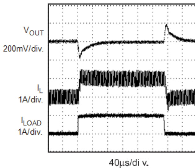
Figure 12. Load Transient
