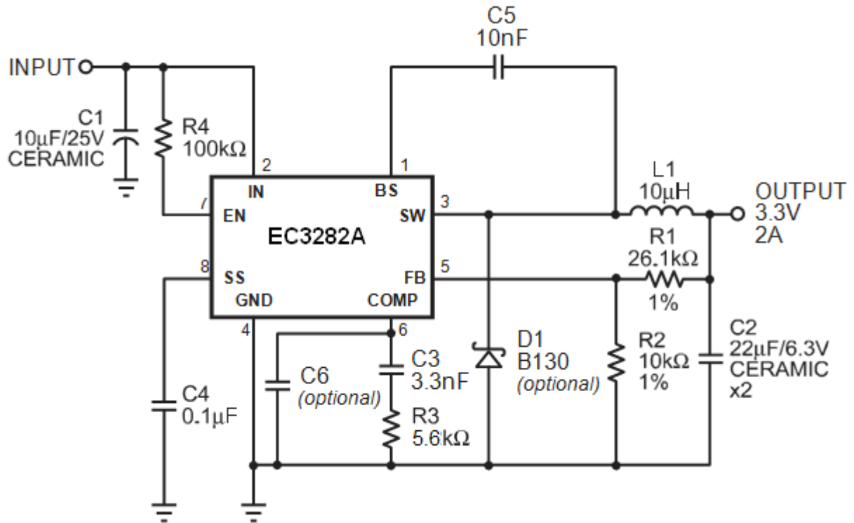
Fig13. EC3282A with 3.3V Output, 22 \mu F/6.3V Ceramic Output Capacitor
