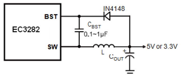
Figure14. Add Optional External Bootstrap Diode to Enhance Efficiency
