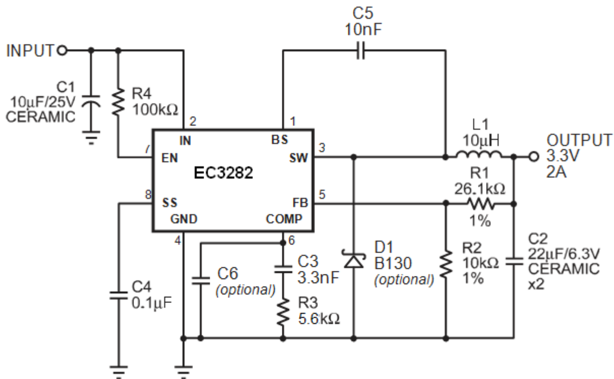
Fig13. EC3282 with 3.3V Output, 22μF/6.3V Ceramic Output Capacitor
