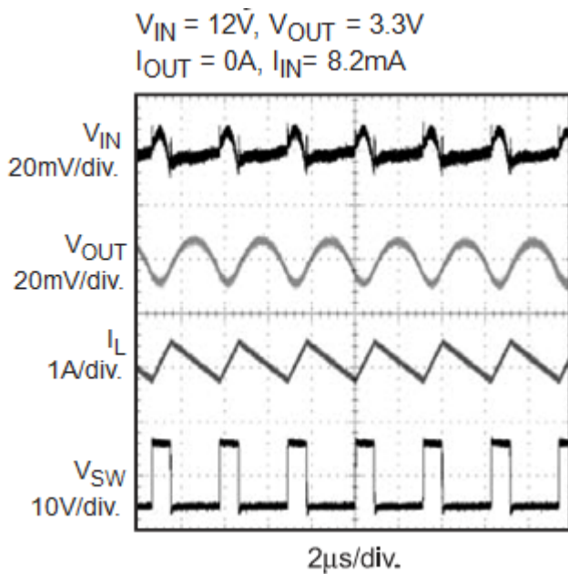
Figure 4. Steady State Test Enable
