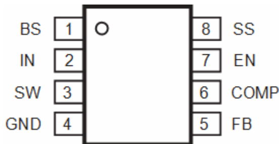
Figure 2 Pin Configuration of EC3282(Top View)
