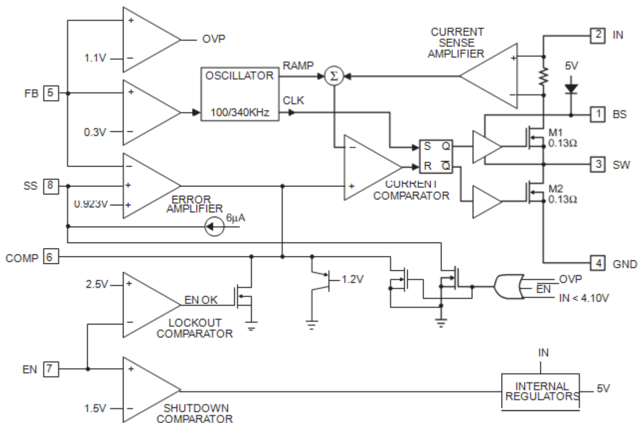
Figure 3 Function Block Diagram of EC3282
