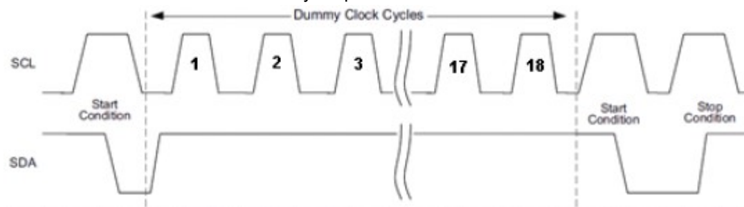
Figure 6: Software Reset
