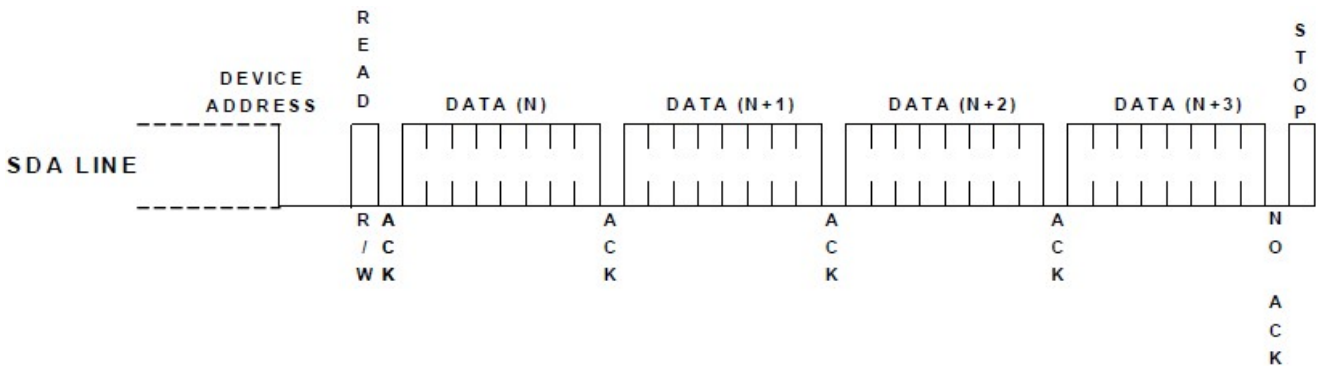
Figure 12: Sequential Read
