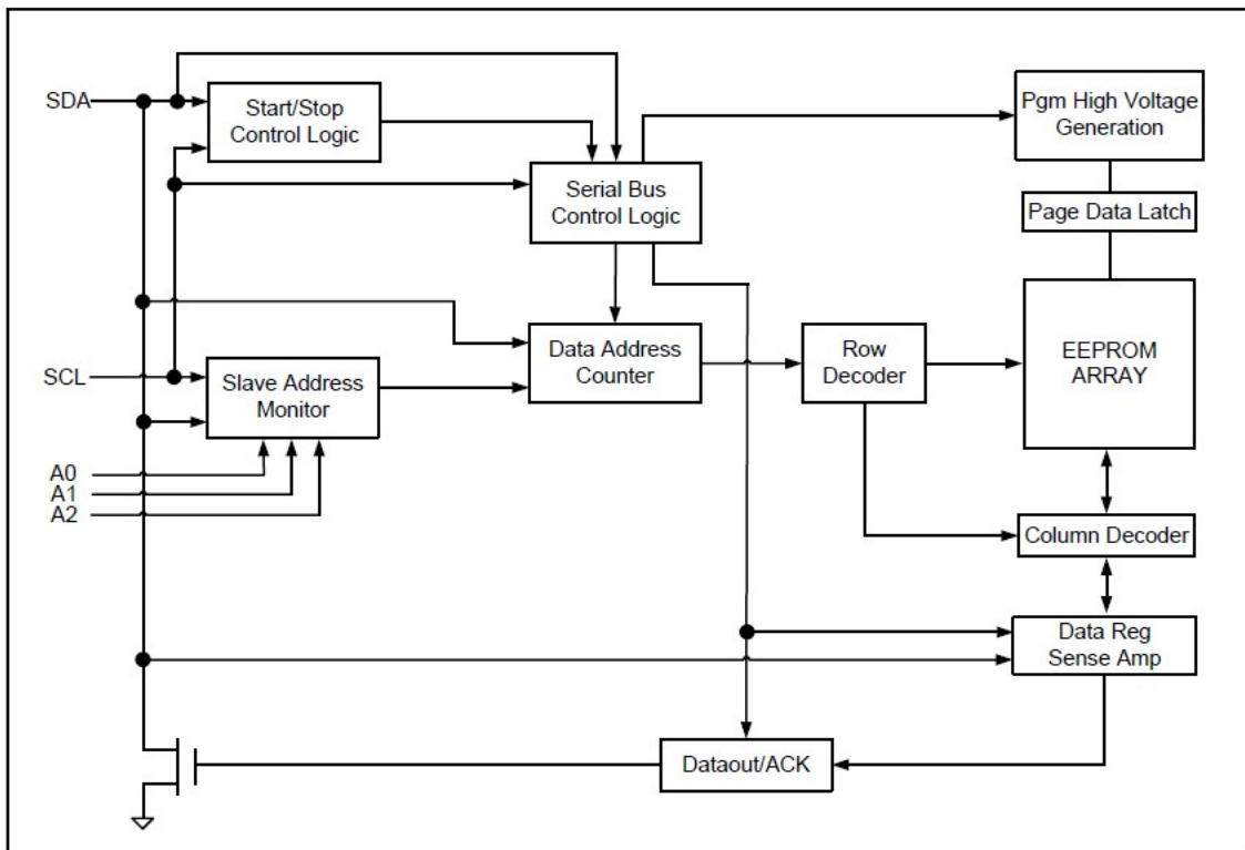
Figure 2: Block Diagram
