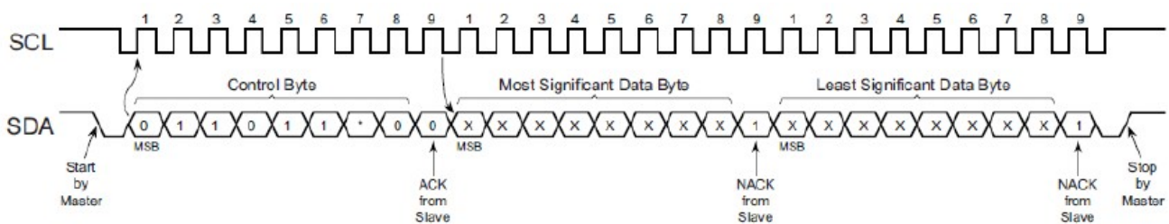
Figure 7: Set Page Address (SPA)
