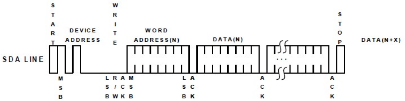
Figure 10: Page Write
