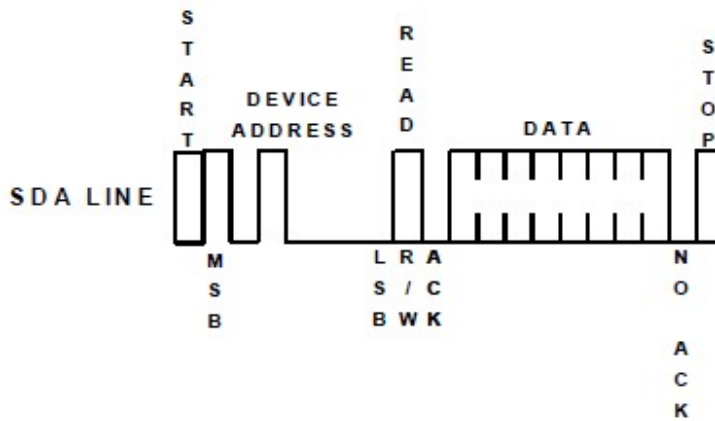
Figure 11: Current Address Read
