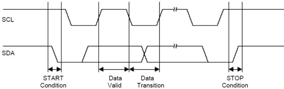
Figure 4: Timing diagram for output ACKNOWLEDGE
