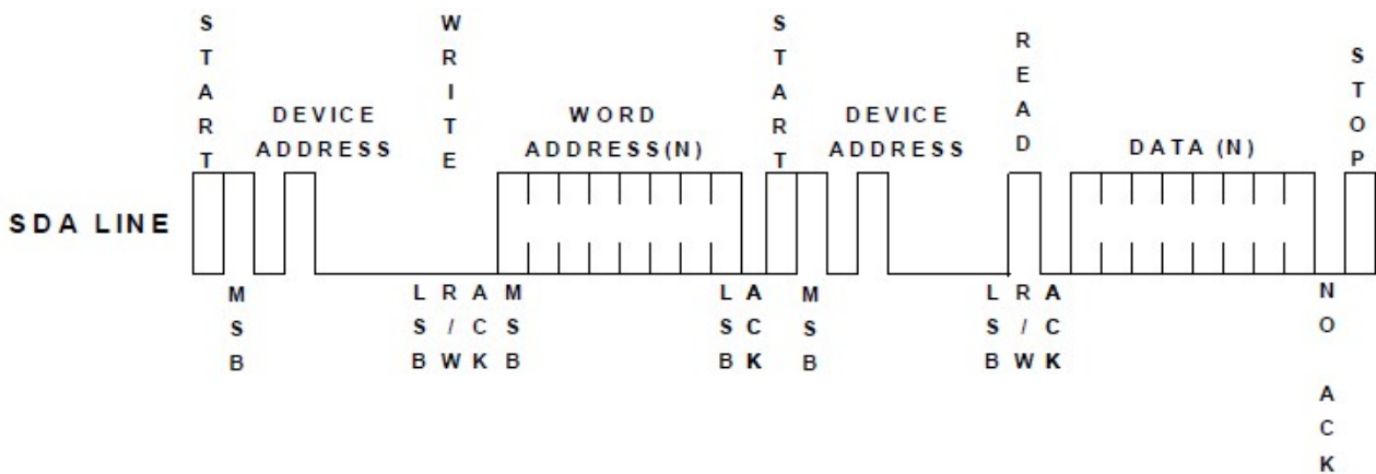
Figure 13: Random Read
