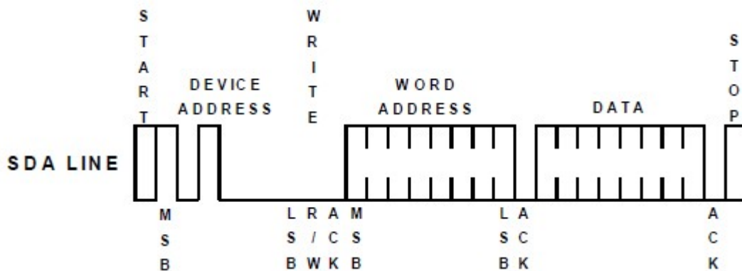
Figure 9: Byte Write
