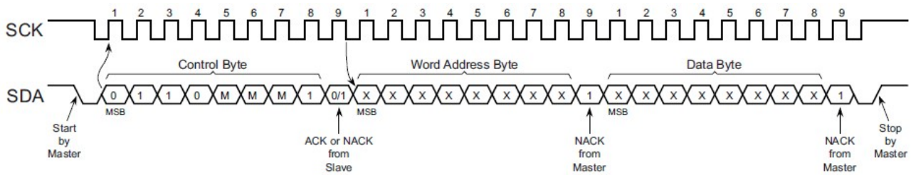
Figure 15: Read RSWP
