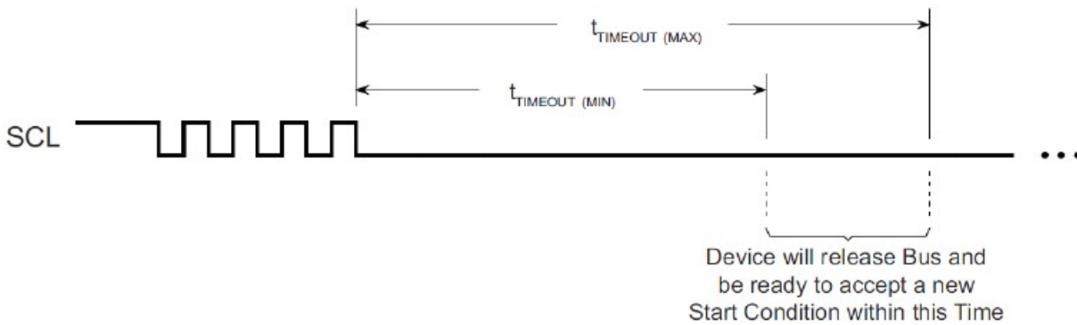
Figure 5: Timeout
