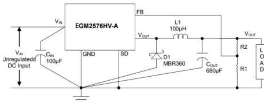
Figure 2 Adjustable Output Voltage Versions
