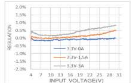
Line Regulation
