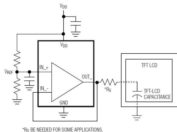
Figure 3. Typical Application Configuration.
