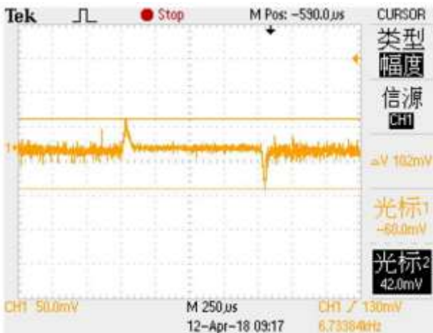
VOUT=3.3V, 1.5A -> 0.2A -> 1.5A load jump
