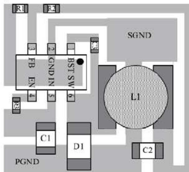
Figure 2: PCB Layout
