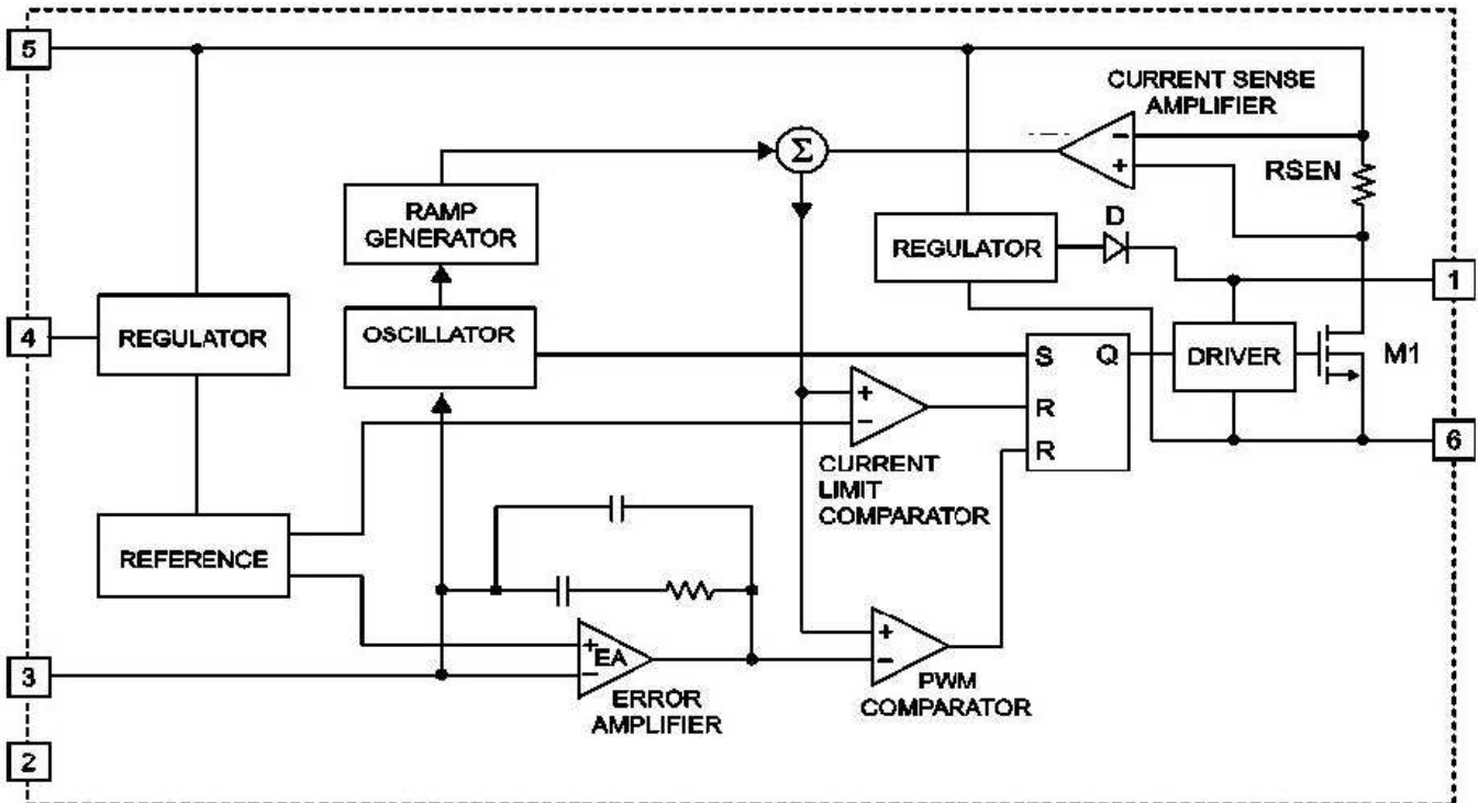
Figure1 Function Block Diagram of EC1466
