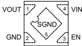
DFN-1x1-4L
