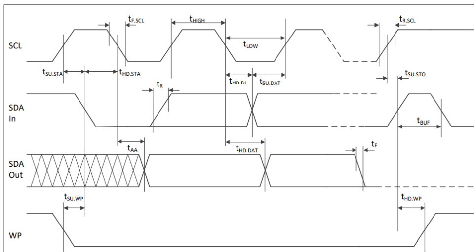
Figure 6-1 Bus Timing
