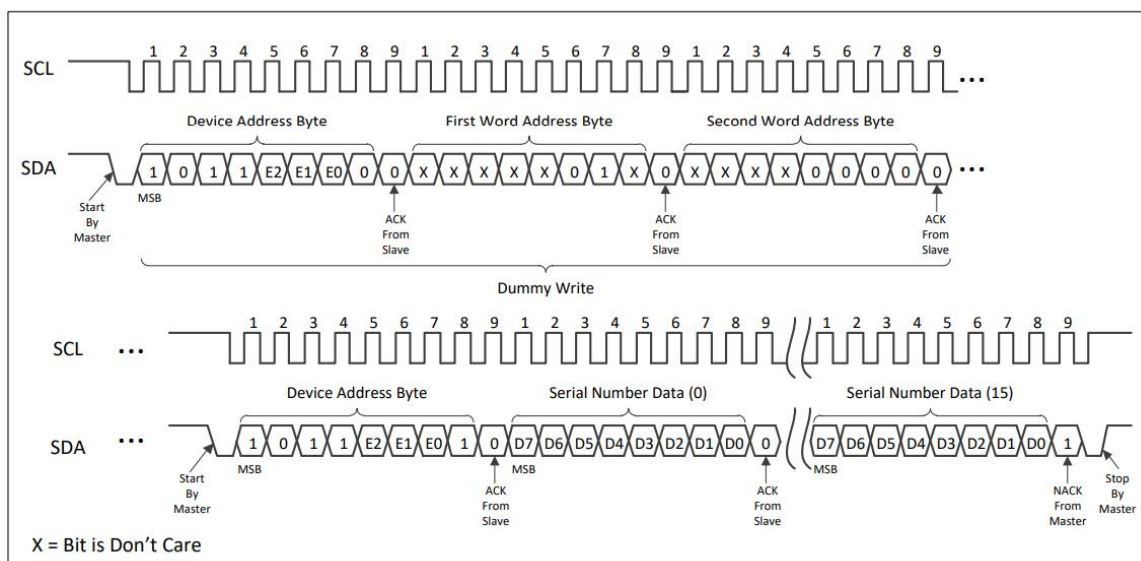
Figure 5–14 Read Unique ID
