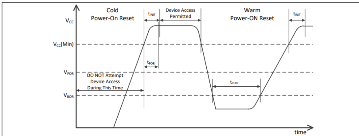
Figure 3–3 Power-up and Power-down Timing
