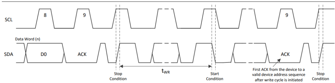
Figure 5–5 Write Cycle Timing
