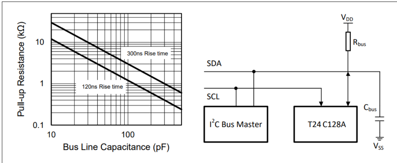
Figure 6–2 Maximum Pull-up Resistance vs. Bus Parasitic Capacitance
