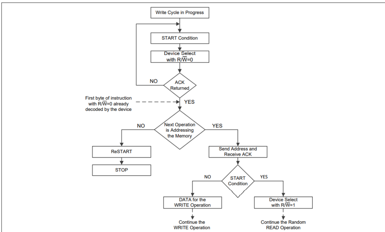
Figure 5–6 Acknowledge Polling Flow Chart
