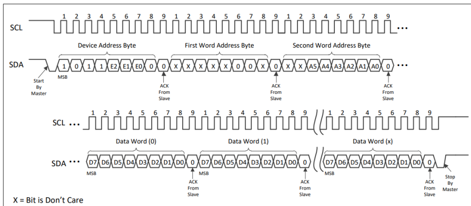
Figure 5–7 Write Identification Page
