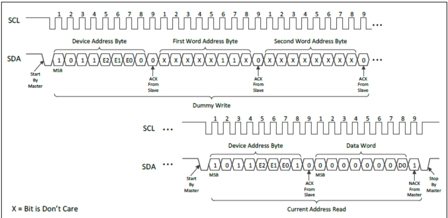
Figure 5–15 Read SWP Bit
