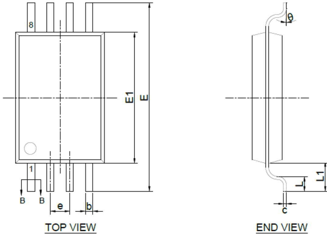
Figure 9-2 8-pad 3.0 x 4.4mm TSSOP Package Outline
