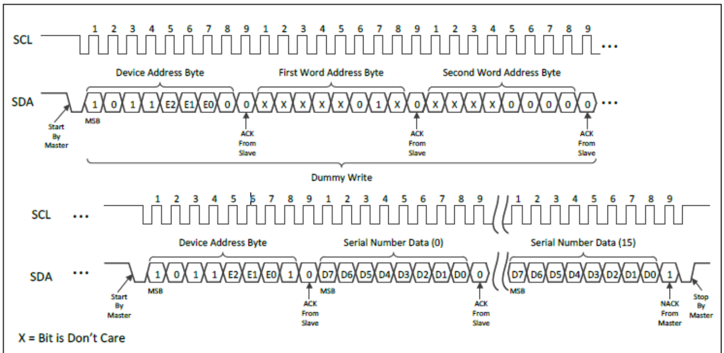
Figure 5–16 Read Unique ID
