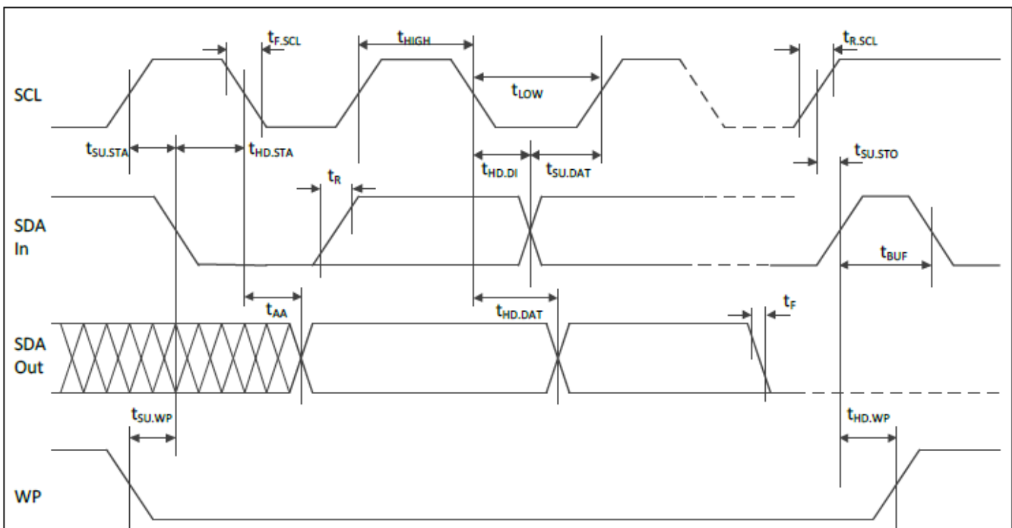
Figure 6-1 Bus Timing
