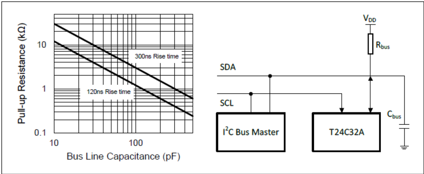
Figure 6–2 Maximum Pull-up Resistance vs. Bus Parasitic Capacitance
