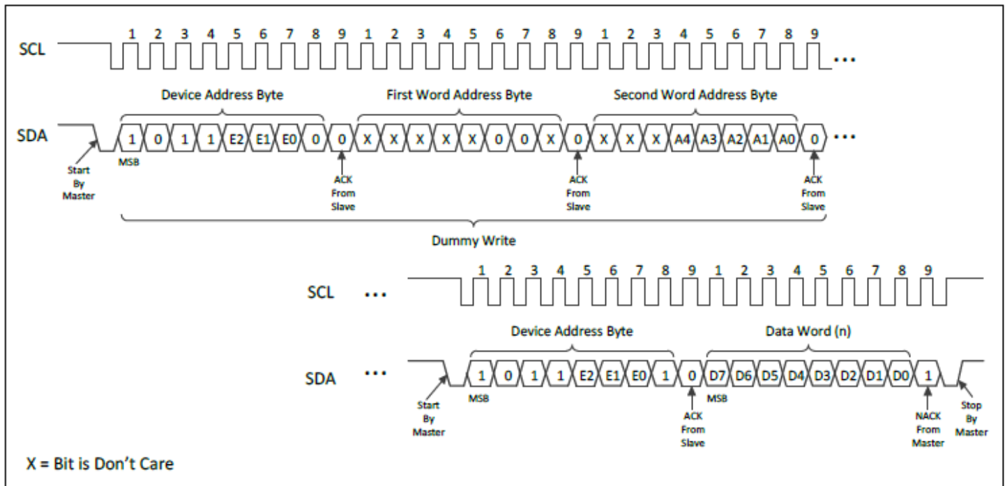
Figure 5–13 Read Identification Page
