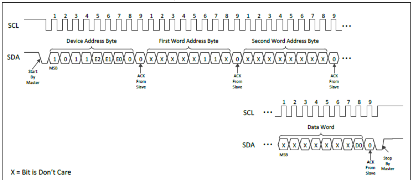
Figure 5-9 Write SWP Bit
