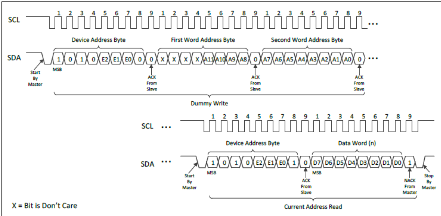
Figure 5–11 Random Read
