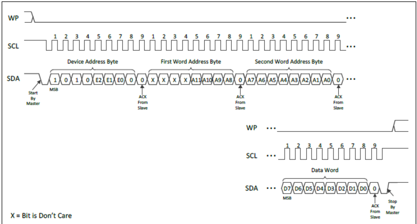
Figure 5–1 Byte Write Operation with Write Protection Pin Set to Low (and SWP bit = 0)
