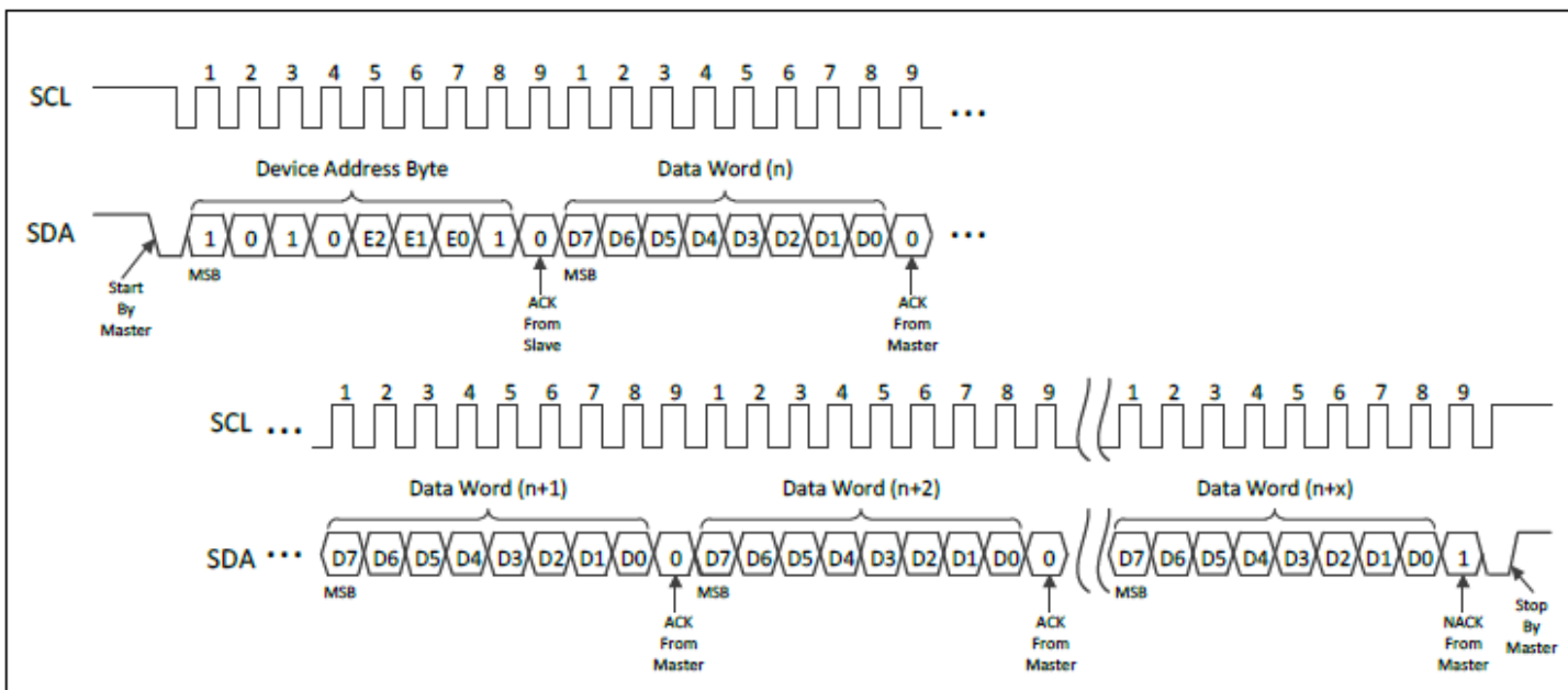
Figure 5–12 Sequential Read
