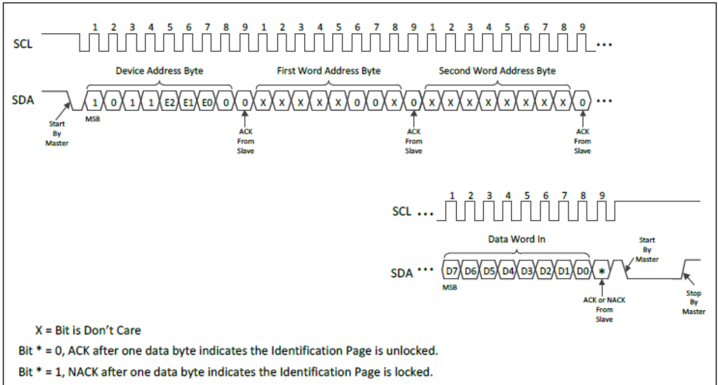
Figure 5–14 Read Lock Status
