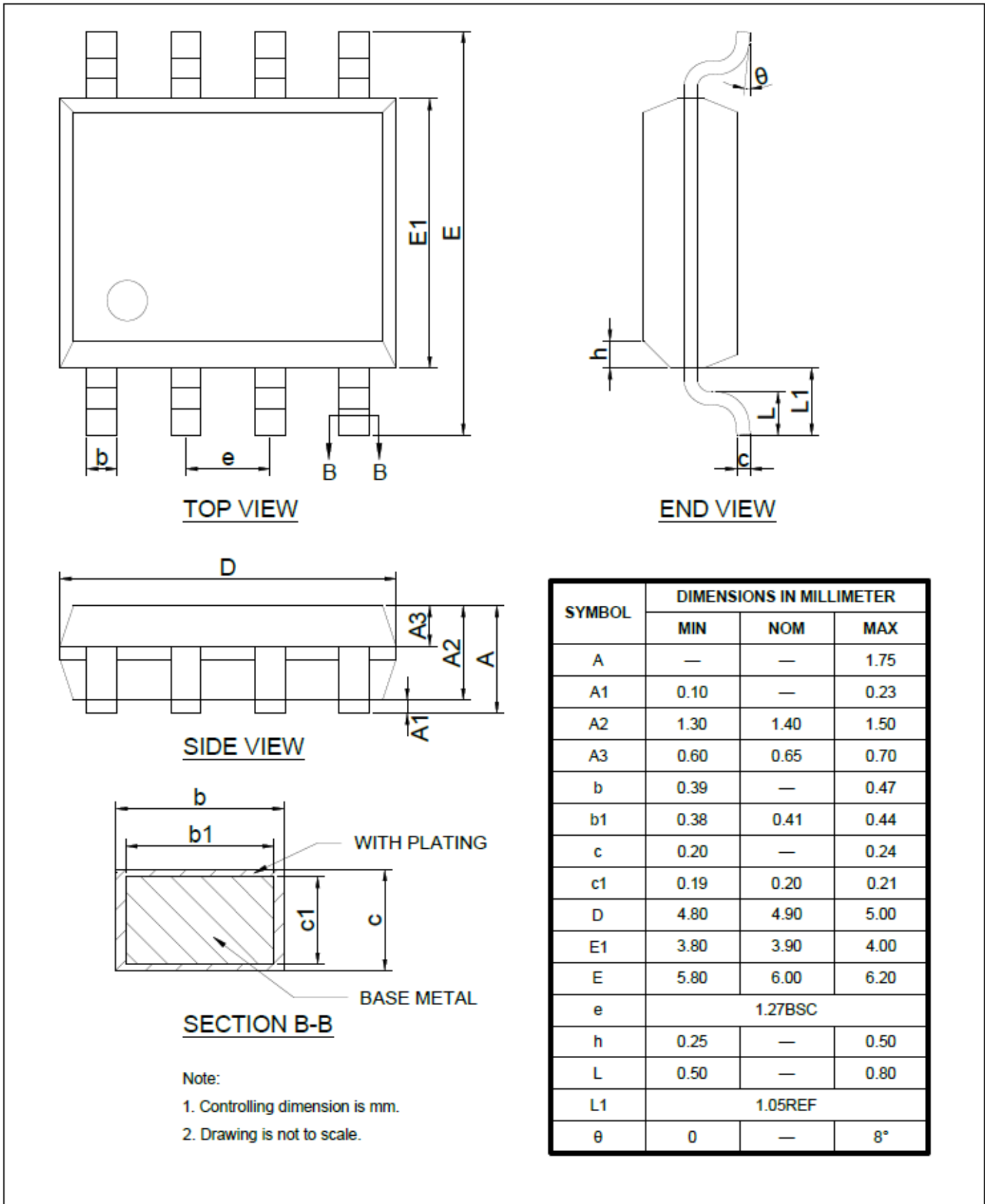
Figure 9-3 8-pad SOP Package Outlin
