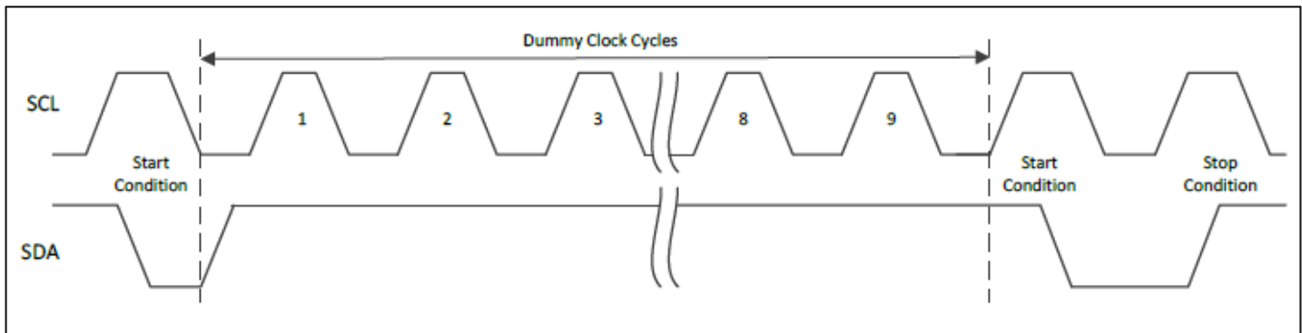
Figure 3–2 2-wire Software Reset
