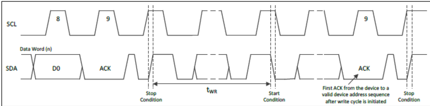
Figure 5-5 Write Cycle Timing
