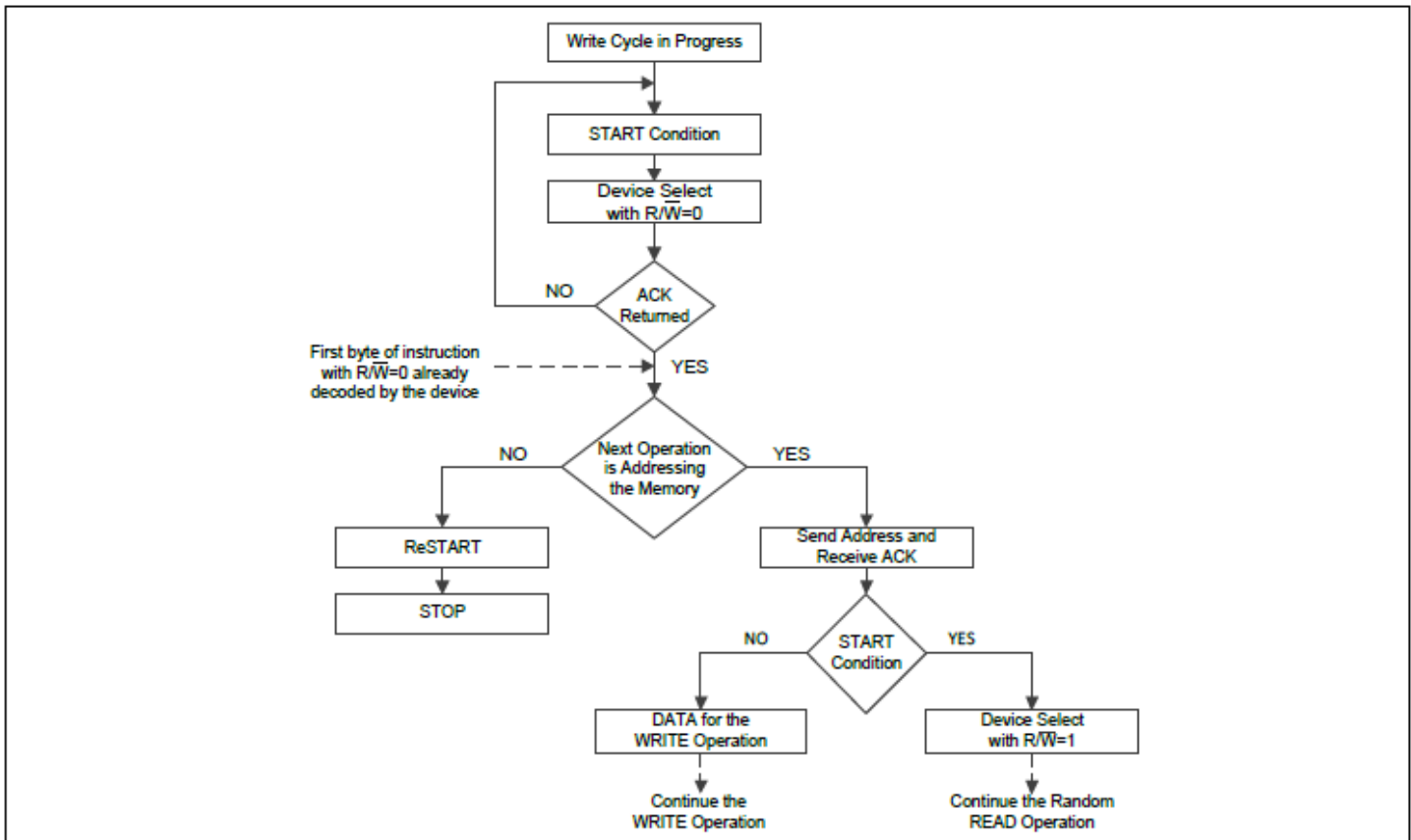
Figure 5-6 Acknowledge Polling Flow Chart
