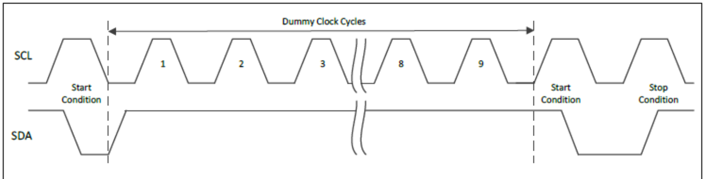
Figure 3–1 Start, Stop, and ACK
