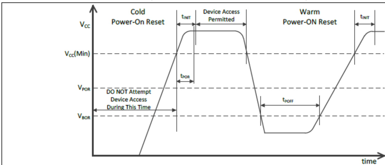
Figure 3–3 Power-up and Power-down Timing
