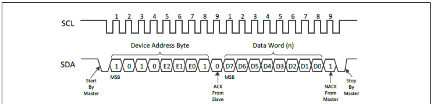
Figure 5–10 Current Address Read
