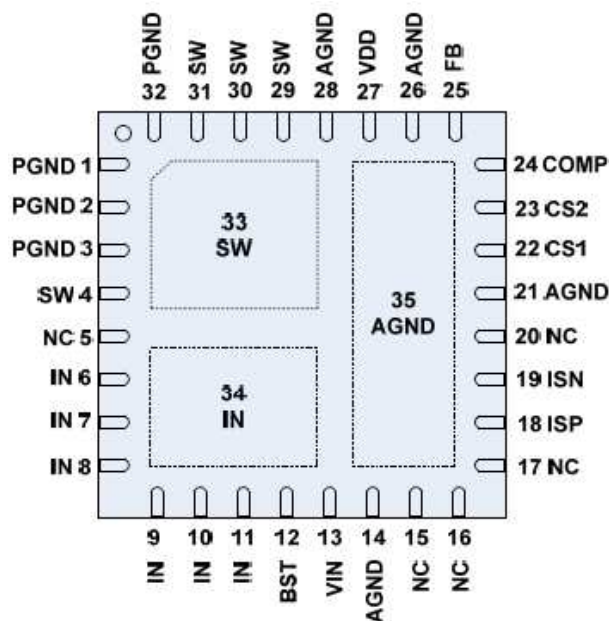
Figure1 Pin Configuration of EC3268A (Top View)
