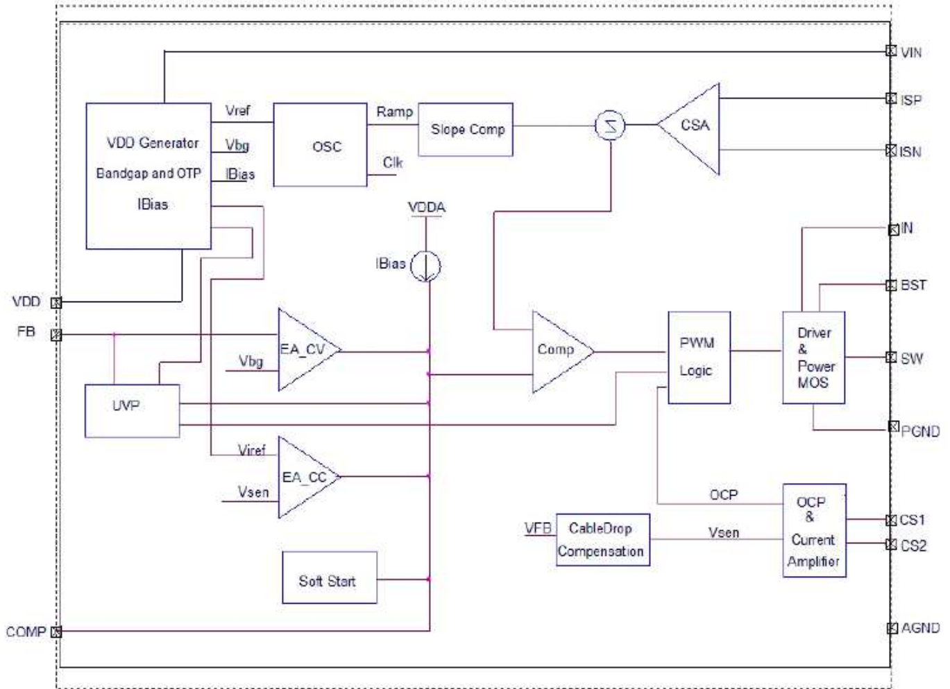
Figure 2 Function Block Diagram of EC3268A
